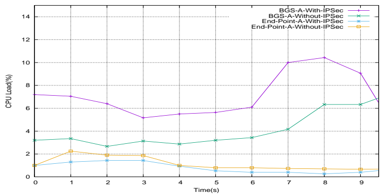
Fig. 9. Performance of SDN security service in term of CPU Load
