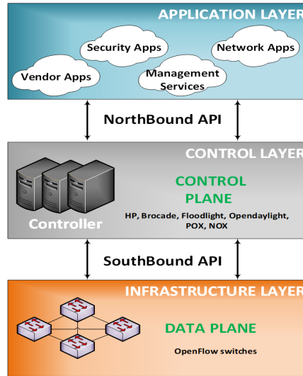
Fig. 1. Architecture SDN
