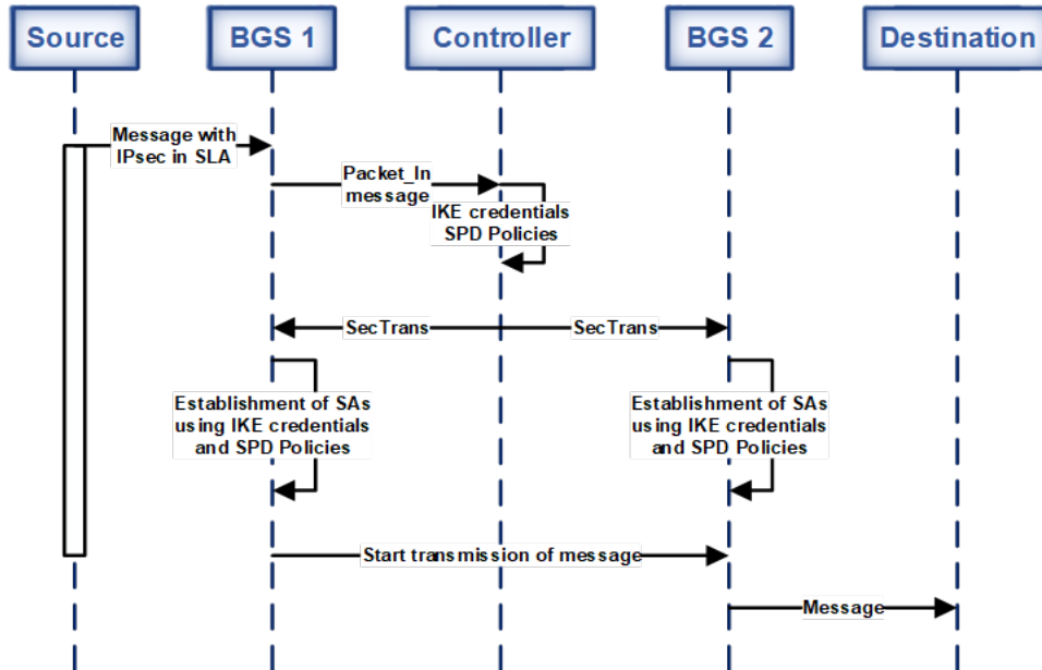
Fig. 4. Flow chart of IPsec service deployment
