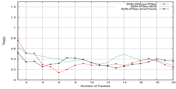
Fig. 8. Performance of SDN security service in term of jitters
