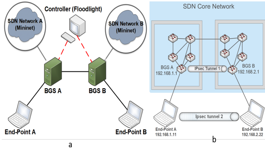
Fig. 5. a. Physical Topology of Testbed. b. Logical Topology of Testbed
