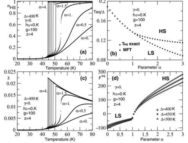
Figure 1. Some features of the model as functions of temperature T and parameter \alpha in mean-field approximation. a,c) Gradual and first-order transitions are depicted for selected values of \alpha and fixed other parameters. The curves shift to the left when \alpha increases and jumps appear in their behaviors. b) The reduced equilibrium temperature T_{eq}/\Delta as function of \alpha obtained by two methods (see text). d) Equilibrium free energy as function of \alpha . The point F_{\alpha=1.05}^{eq} = 0 [49] is the onset of first-order transitions for selected values of \Delta (400, 450, and 500 K). n_{HS} and m are solutions at thermodynamic equilibrium, that is, corresponding to the minimum of the free energy. Other parameters values are written in the panels.
