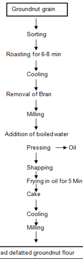
Fig. 2. Process flow diagram for roasted defatted groundnut flour Source: Modified from Adjou et al., [17]
